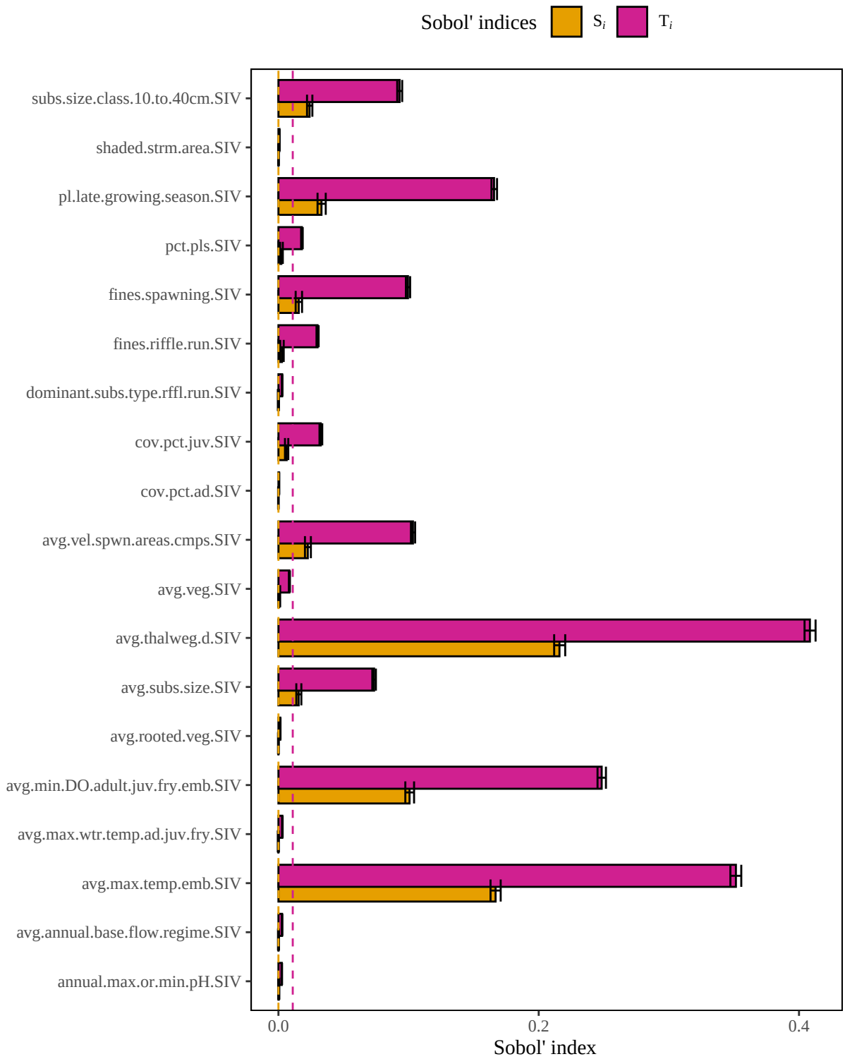
Figure 3. Results of a sensitivity analysis for the cutthroatRivGenMt15CMt5m model based on the original author-specified model outlined in Hickman and Raleigh (1982). Dashed lines represent baseline numerical approximation error for S_i and T_i ( i.e. , dummy variables).
